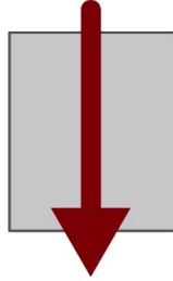
down
