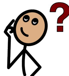
why
