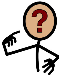
who
